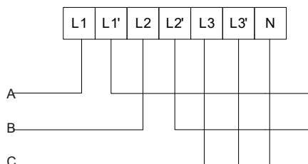
Fig 4 Three phase four lines direct connect
