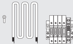
Cable harness, voltage terminals and earth connection
